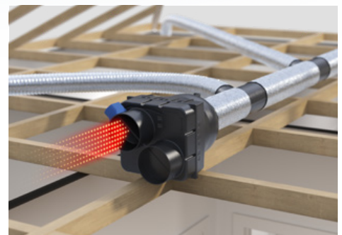
The fan enclosure moves air through the system
