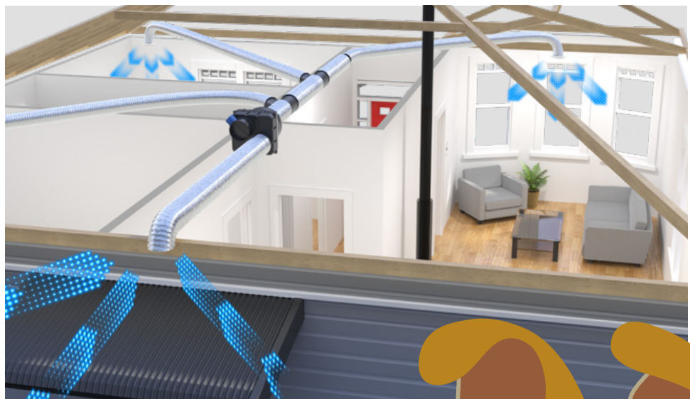
Summer Kit draws fresher, cooler air inside
