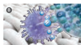
Hydroxyl radicals take hydrogen away from pollutants
